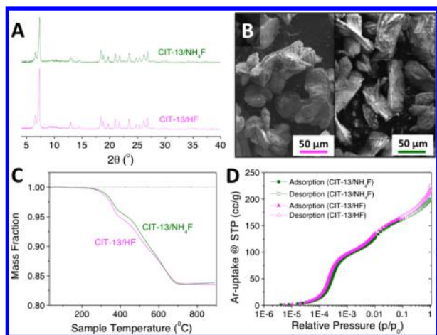
Figure 6. Comparison of the HF and \text{NH}_4\text{F} protocols for preparing CIT-13. (A) XPD patterns, (B) SEM micrograph images of CIT-13 resulting from the HF (left) and the \text{NH}_4\text{F} (right) protocols, (C) TGA profiles, and (D) argon adsorption and desorption isotherms at 87.45 K.
