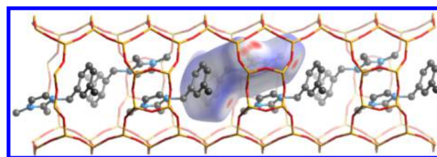
Figure 10. 14-ring channel of CIT-13 (along the z axis) viewed down the 10-ring channel ( y axis), showing the Hirshfeld surface of one OSDA and the arrangement of OSDAs at the intersections of the channels.
