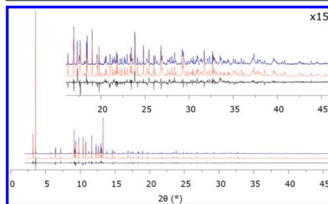
Figure 7. Observed (blue), calculated (red), and difference profiles (black) for the Rietveld refinement of as-prepared CIT-13.
