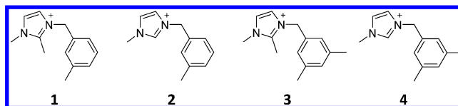
Figure 2. Organic structure-directing agents (OSDAs) used in this study to produce CIT-13 in a germanosilicate system and fluoride medium.
