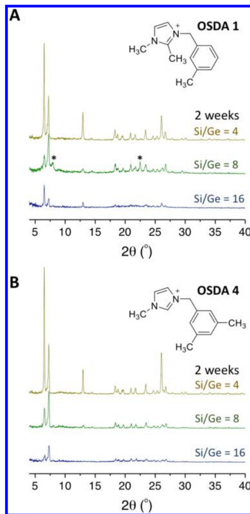
Figure 4. XPD patterns of the samples resulting from different Si/Ge ratios in the gel with (A) OSDA 1 and (B) OSDA 4 for gel compositions x/(x + 1) \text{ SiO}_2:1/(x + 1) \text{ GeO}_2:0.5 \text{ (OSDA)OH}:0.5 \text{ HF}:10 \text{ H}_2\text{O} where x is the gel Si/Ge ratio. Asterisks (*) denote impurity peaks.
